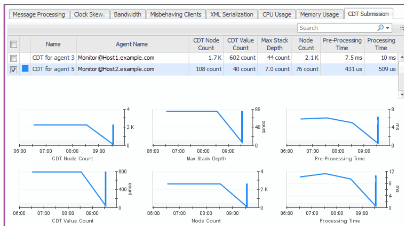
Figure 16. CDT Submission tab
