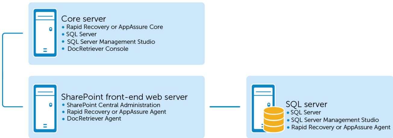
Figure 4. Simple DocRetriever configuration with separate SQL Server
