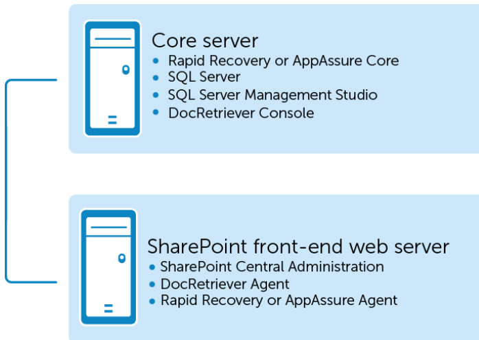
Figure 1. DocRetriever in standard mode, two servers
